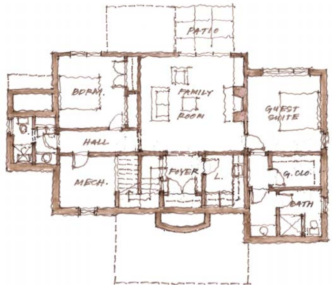
FINISHED BASEMENT PLAN
