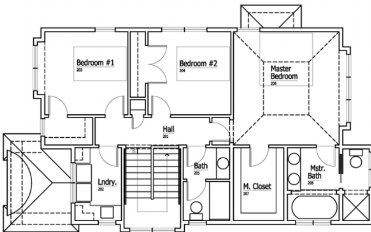
Second Floor Plan 1,069 SF
