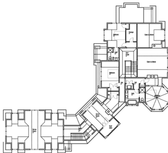
Second Floor Plan 3,172 SQ. FT.
