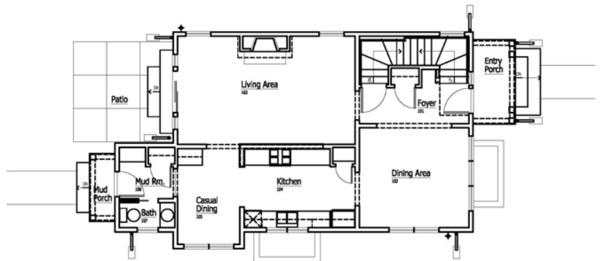
First Floor Plan 955 sf.
