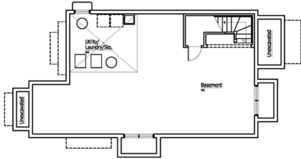
Basement Plan 677 sf.
